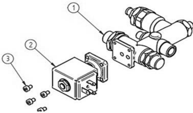
Water inlet assembly
