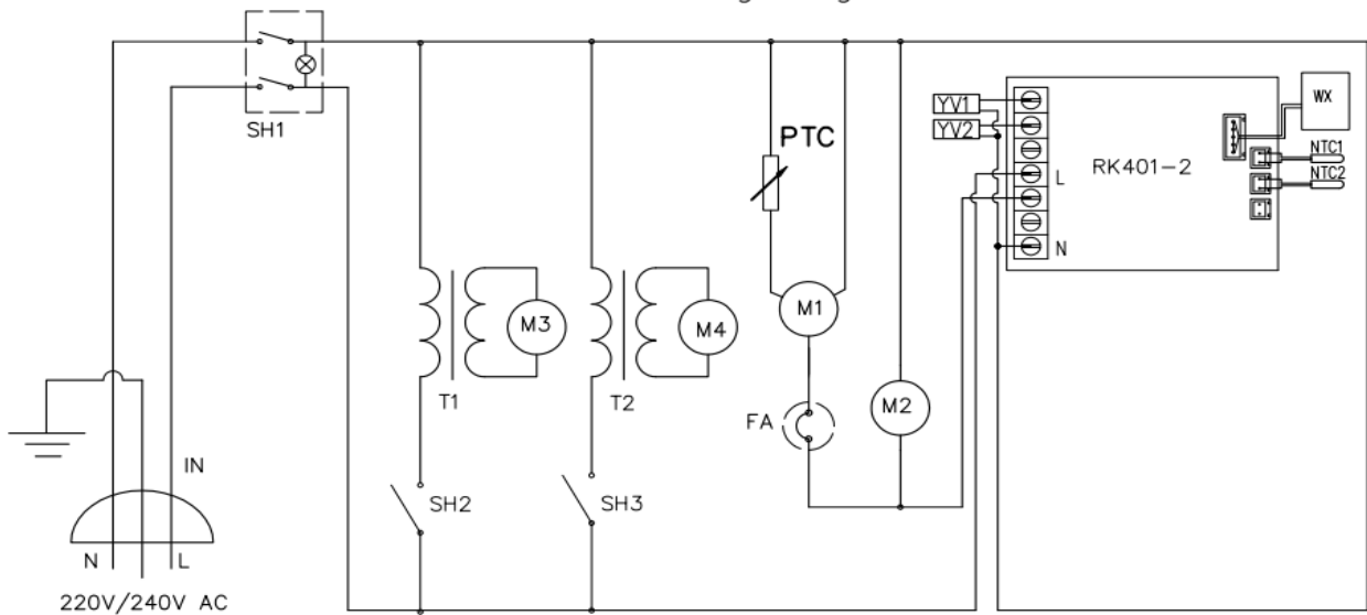
Electric Wiring Diagram
