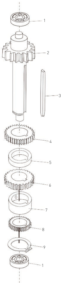
Figure 3: Gear axle assembly
