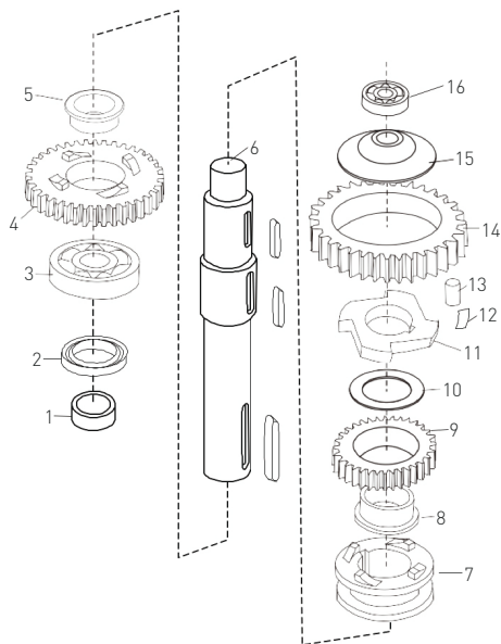
Figure 2: Axle assembly
