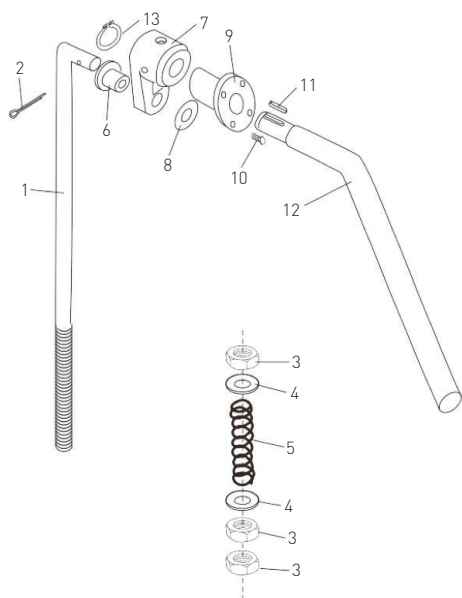
Figure 5: Bowl lift up assembly
