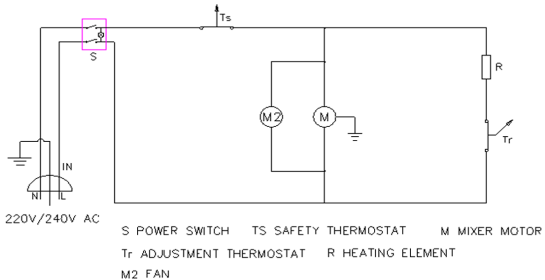
Electric Wiring Diagram
